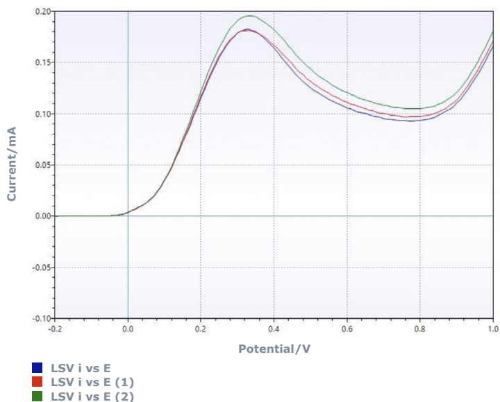
IGSB04192 – Linear sweep voltammogram 0.5 mM uric acid in basic aqueous solution.
